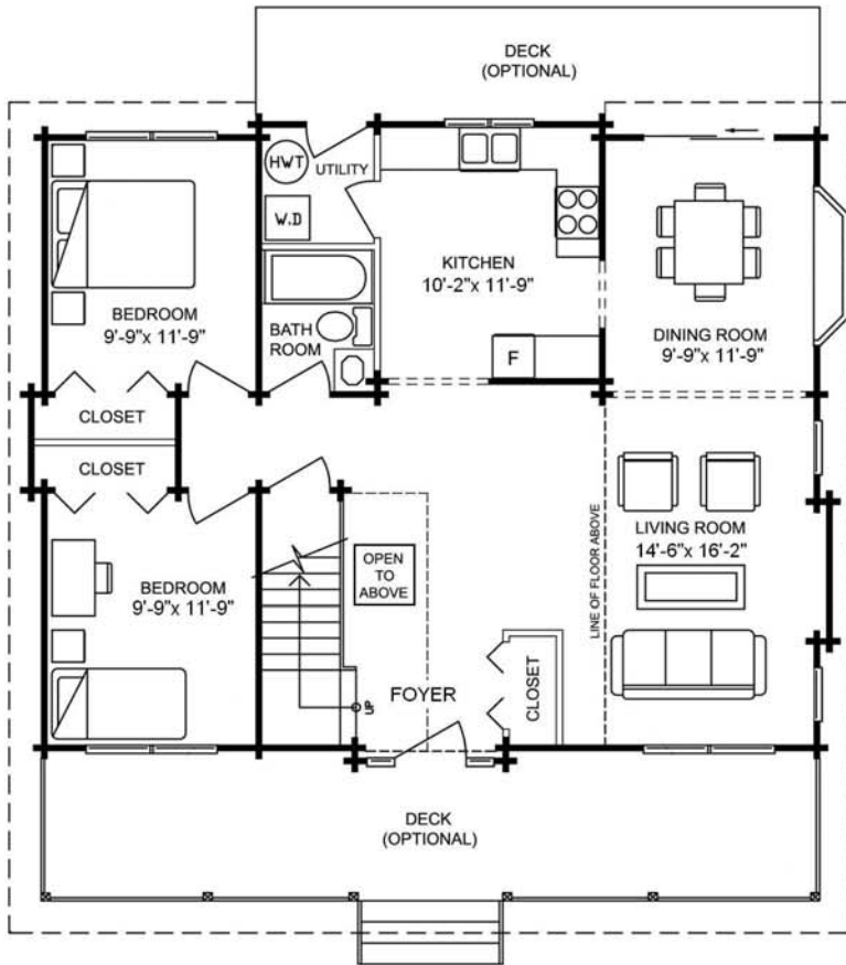
MAIN FLOOR PLAN 1069 sq. ft. (99.27 sq. m.)
