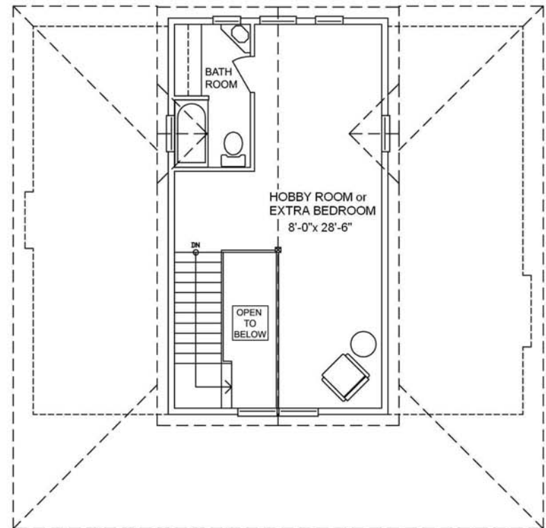
SECOND FLOOR PLAN 383 sq. ft. (35.6 sq. m.)
